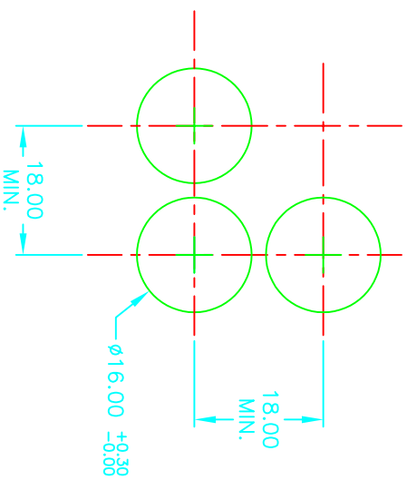
RECOMMENDED PANEL MOUNTING SCALE 1:1
